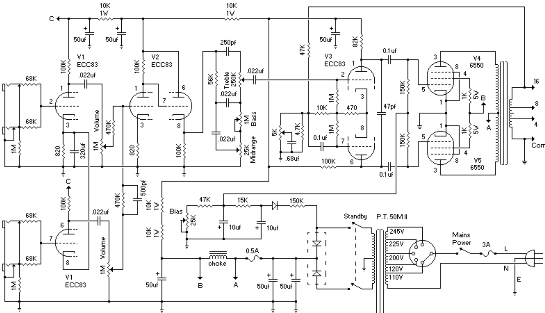
Marshall Amplifier Model # 1986 Bass MK II Drawn By: Joe Piazza 1 / 13 / 97
