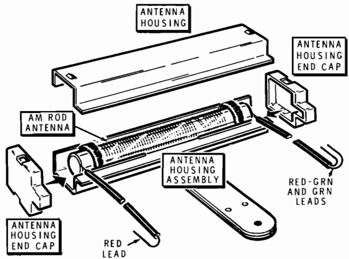
Detail 3-8C
