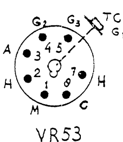
VALVE BASES FROM UNDERSIDE
