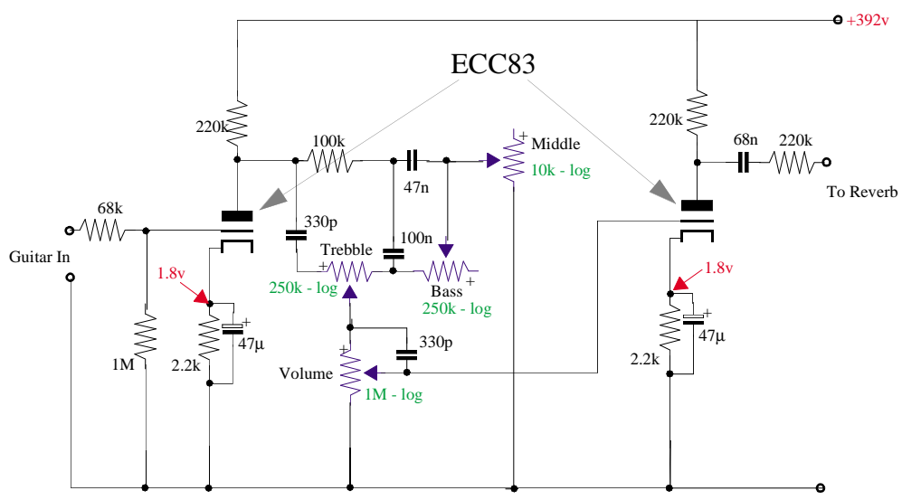
Orange Preamp Section - Channel II
