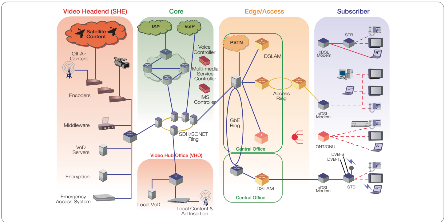
▶ Figure 7. Network Architecture.
