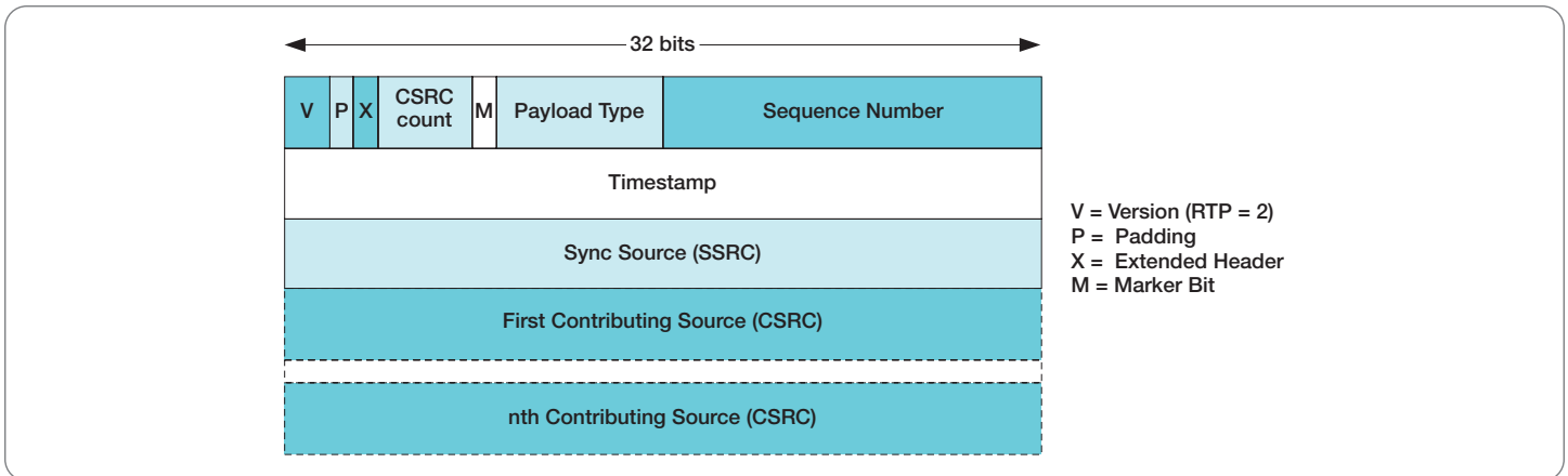
▶ Figure 5. RTP Headers.
