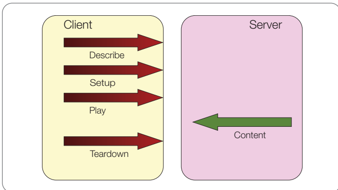
▶ Figure 6. RTSP Protocol.
