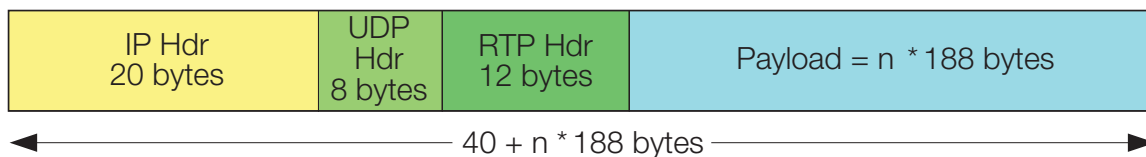
► Figure 4. IP/UDP/RTP Packets.
