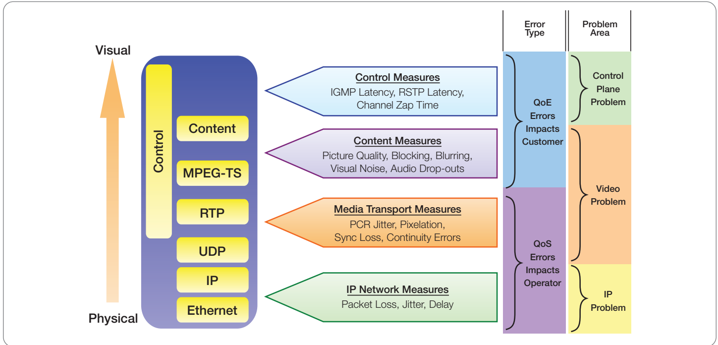
▶ Figure 11. Physical Layer and Protocol Stack Problems.
