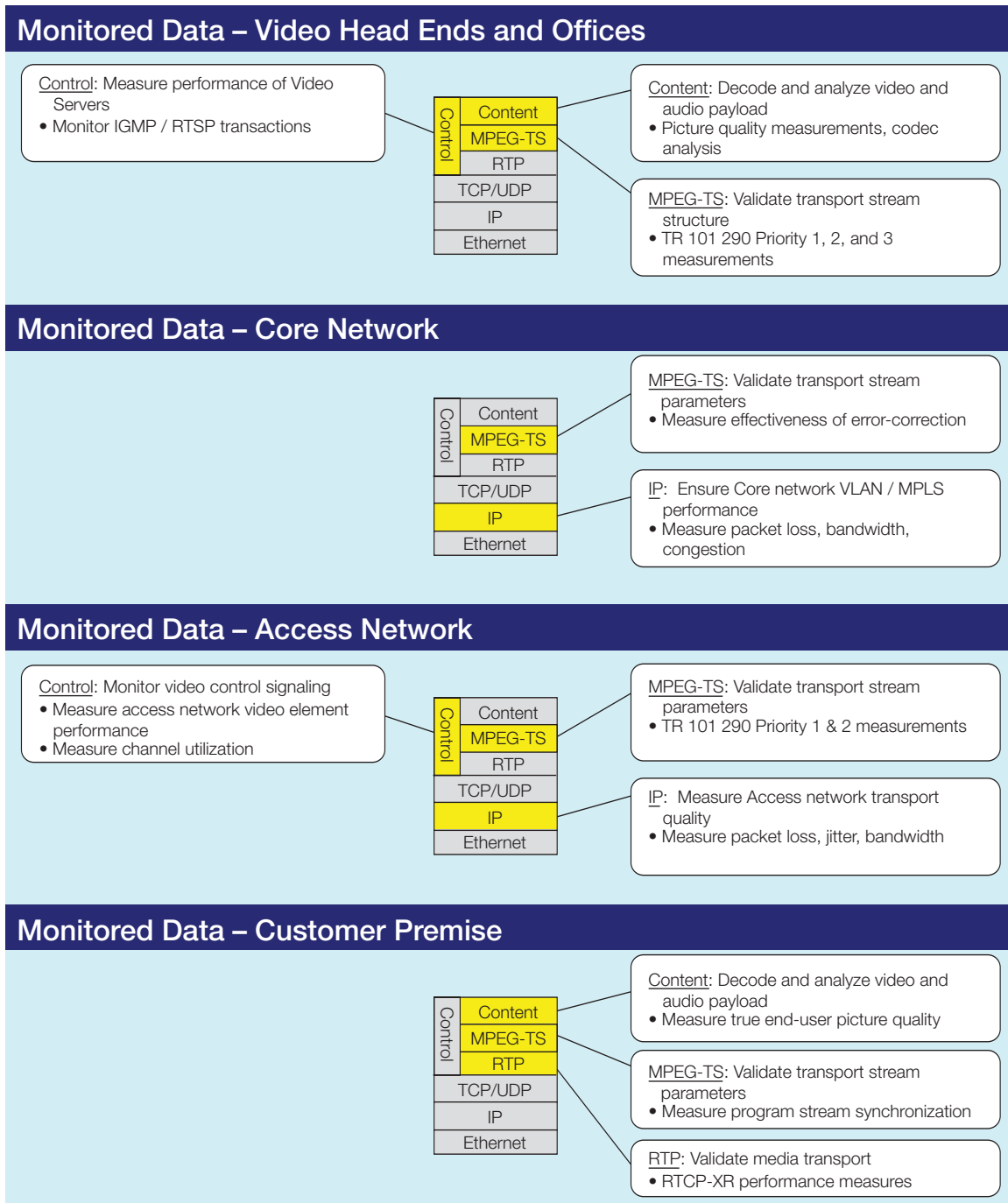
▶ Figure 15. Examples of Multi-Layer Test Points.
