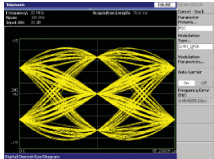
Figure 3-16. Eye diagram display showing a PDC signal.
