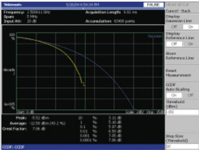
Figure 3-21. CCDF measurement.
