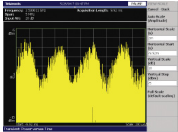
Figure 3-9. Power vs. Time display.
