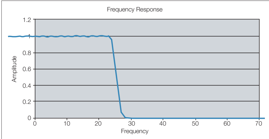
Figure 2-15. Frequency response of a lowpass filter.
