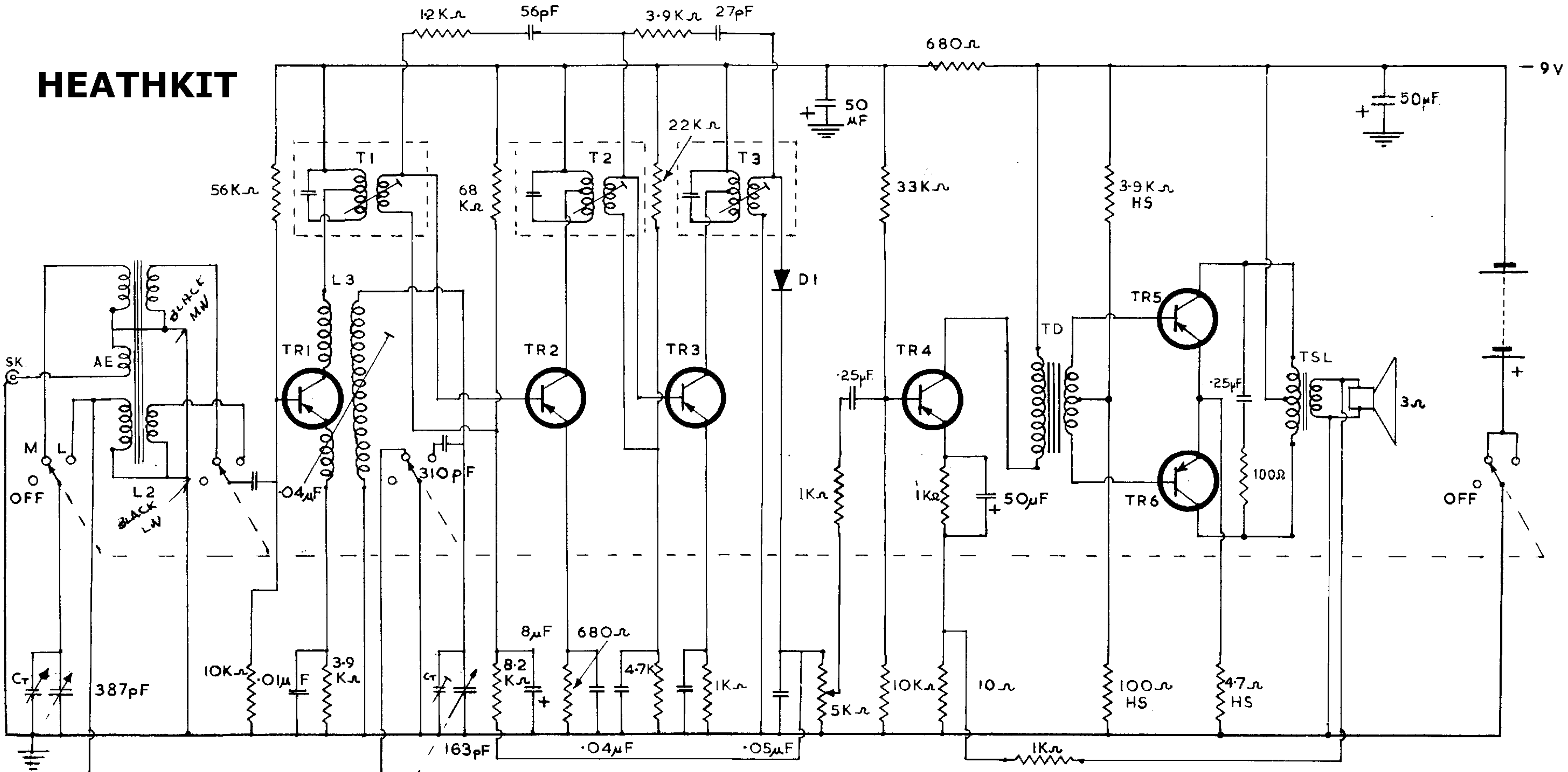
CIRCUIT FOR TRANSISTOR RECEIVER, MODEL UXR-1.
