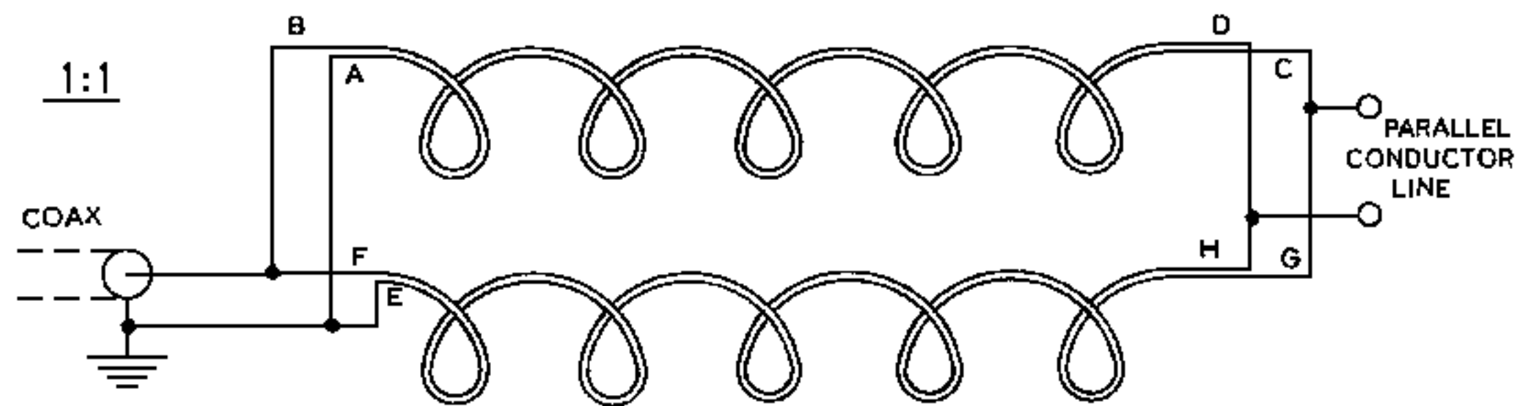
SCHEMATIC HEATHKIT BALUN COIL MODEL B-1
