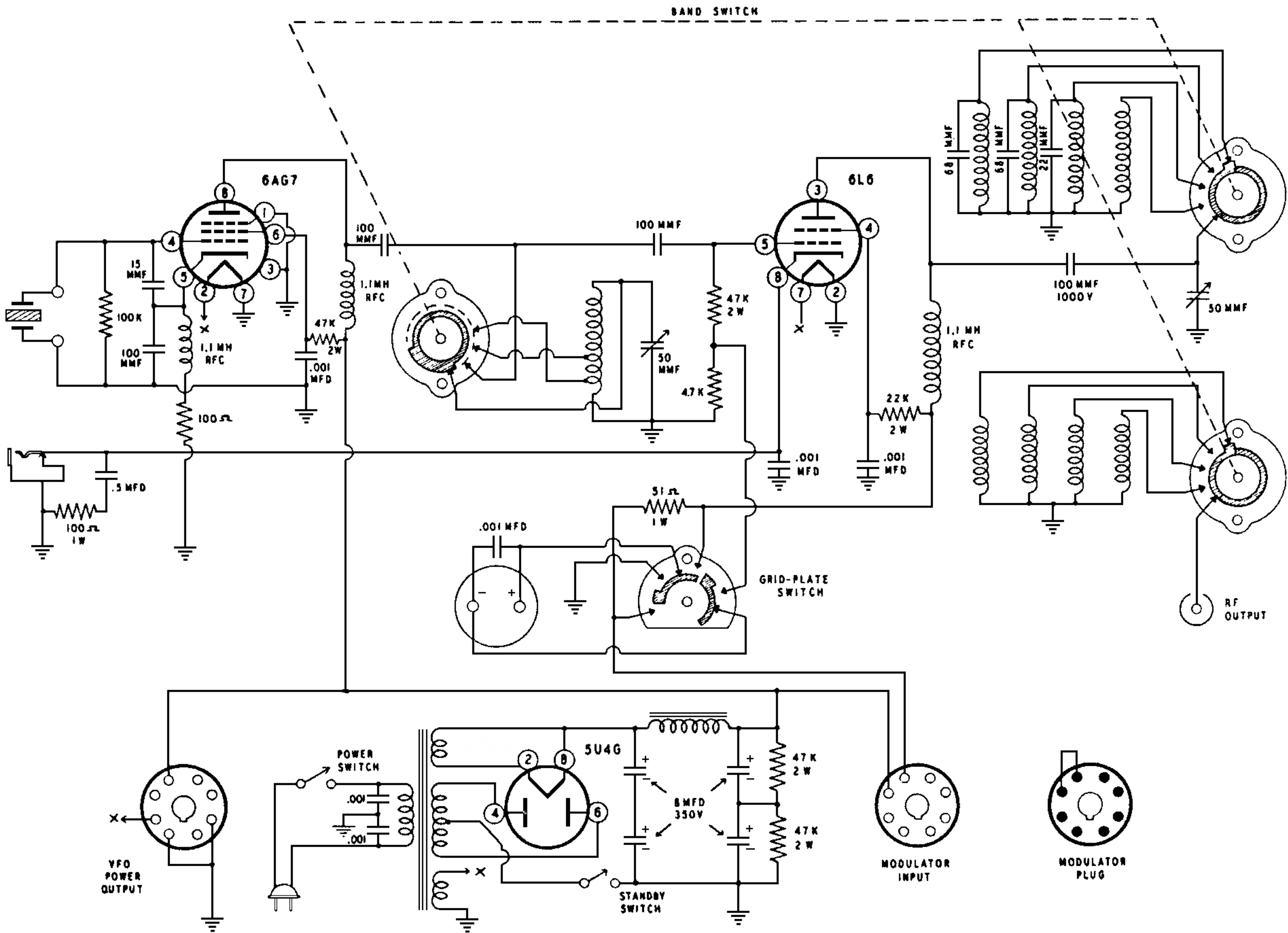
HEATHKIT AMATEUR TRANSMITTER MODEL AT-1
