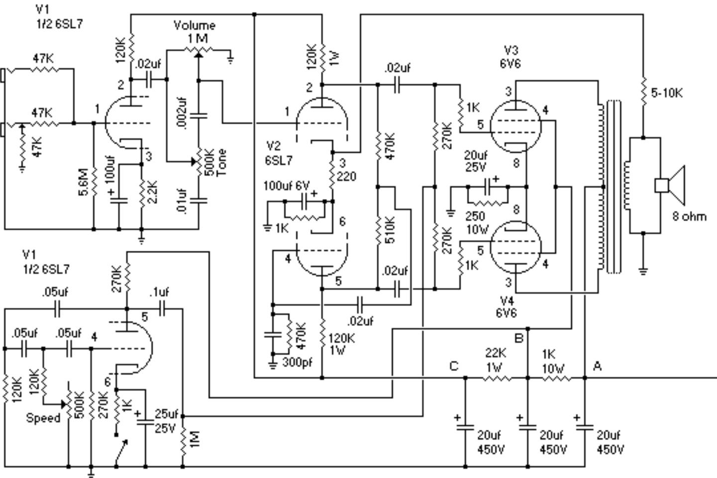
Ampeg Jet Amplifier Model J-12-B (6V6 version) Drawn by: Joe Piazza 12/06/96
