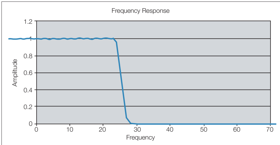
Figure 2-15. Frequency response of a lowpass filter.
