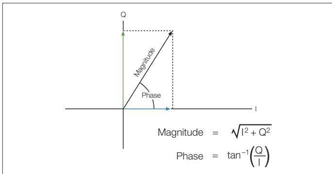
Figure 2-33. Vector representation of magnitude and phase.
