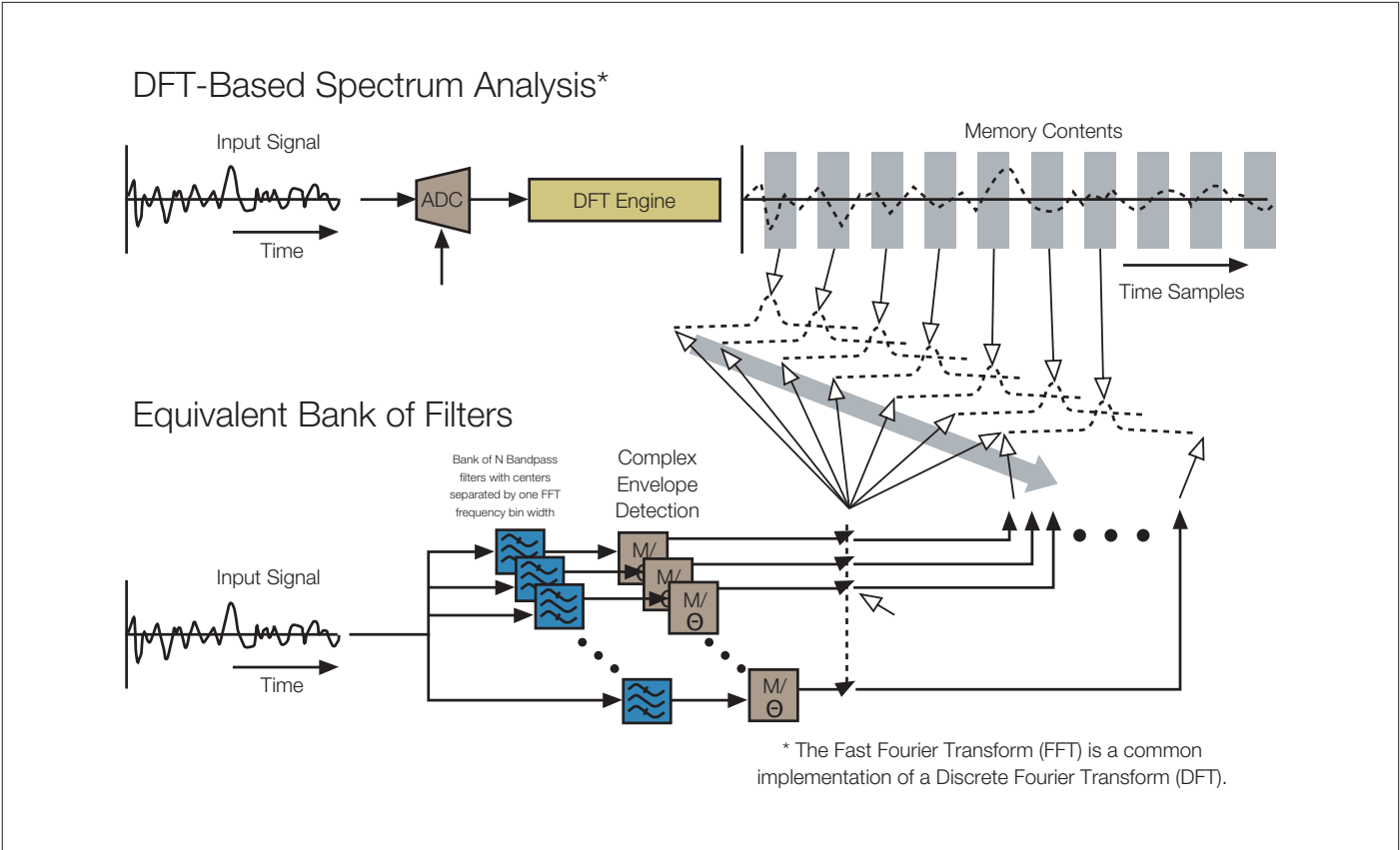
Figure 2-5. A DFT-based Spectrum Analyzer and an equivalent implementation using a bank of bandpass filters.
