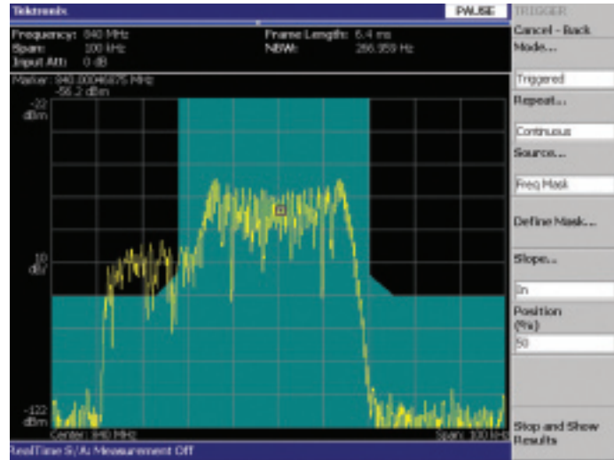
Figure 2-32. One frame of the spectrogram showing the trigger event where the transient signal breaks the boundary of the frequency mask.
