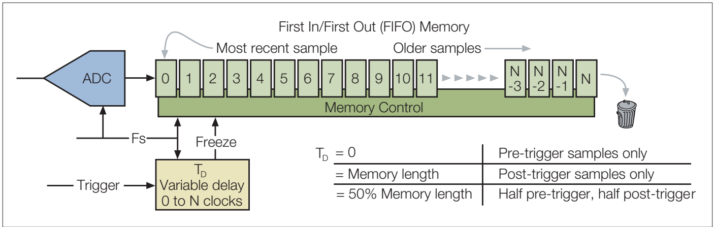
Figure 2-28. Triggering in digital acquisition systems.
