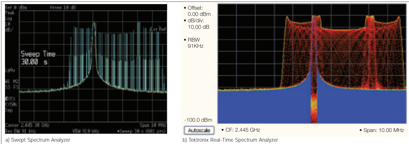
Figure 2-20 a, b. Comparison (a), Swept Spectrum Analyzer MaxHold trace after 120 seconds and (b), Tektronix Real-Time Spectrum Analyzer with DPX bitmap MaxHold trace after 20 seconds.
