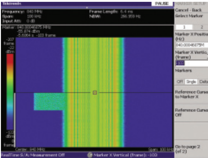
Figure 2-31. Spectrogram showing a transient signal adjacent to the carrier. The cursor is set to the trigger point, so pre-trigger data is displayed above the cursor line, and post-trigger data is displayed below the cursor line. The narrow white line at the left of the blue area denotes post-trigger data.
