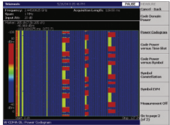
Figure 3-20. Codogram measurement of W-CDMA compressed mode.
