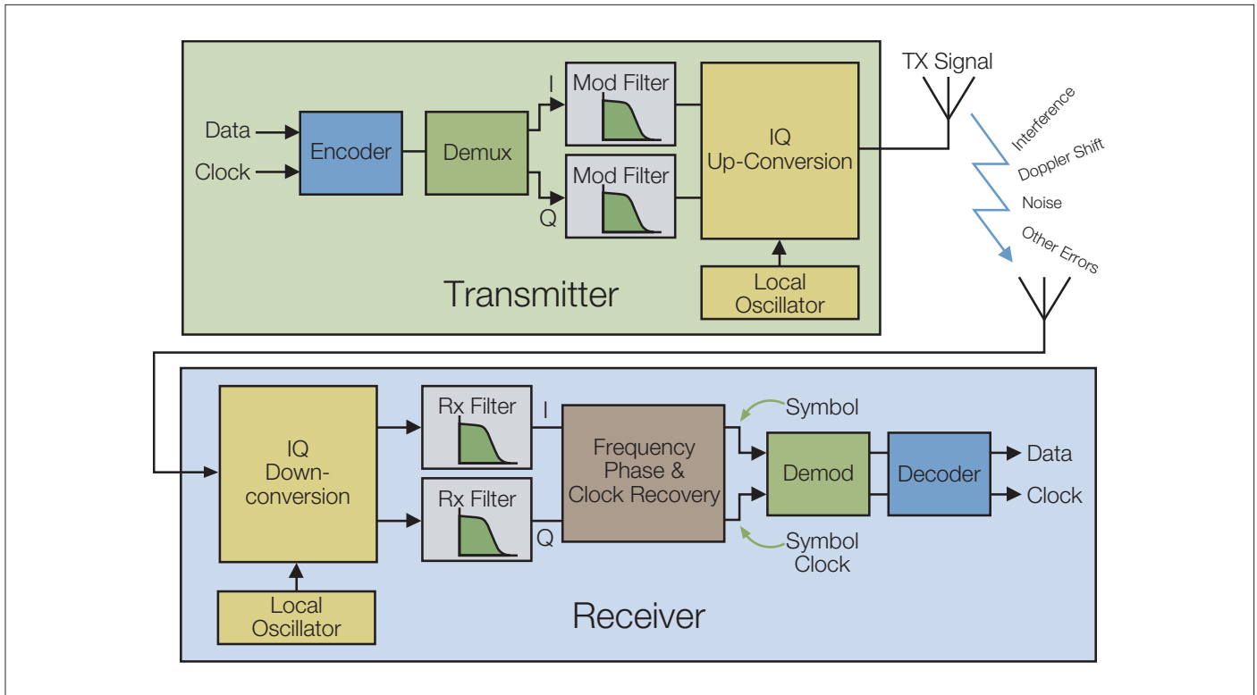
Figure 2-34. Typical digital communications system.
