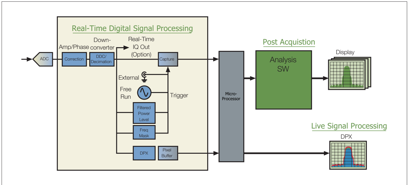
Figure 2-2. Real-Time Spectrum Analyzer Digital Signal Processing Block Diagram.
