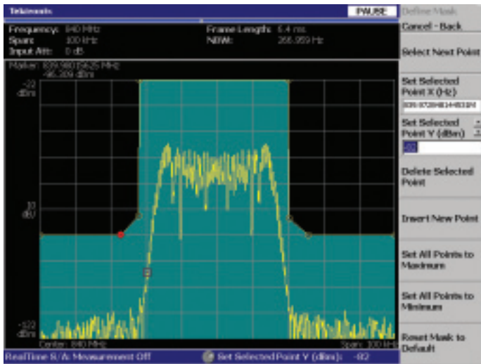
Figure 2-30. Frequency mask definition.
