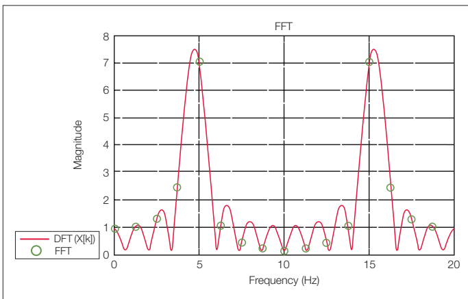
Figure 2-13. FFT of x(n) , length of FFT = N = length of x(n) .
