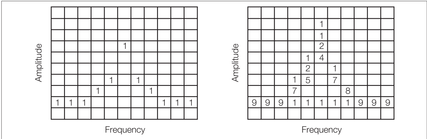
Figure 2-21. Example 3-D Bitmap Database after 1 (left) and 9 (right) updates. Note that each column contains the same total number of "hits."
