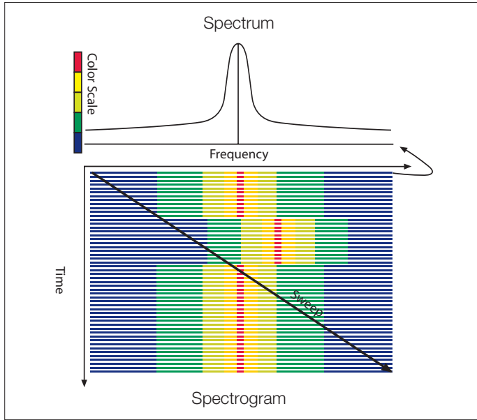
Figure 2-6. Spectrum, Spectrogram and Sweep.
