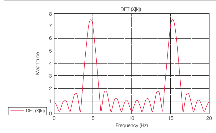
Figure 2-12. DFT of x(n) evaluated continuously.
