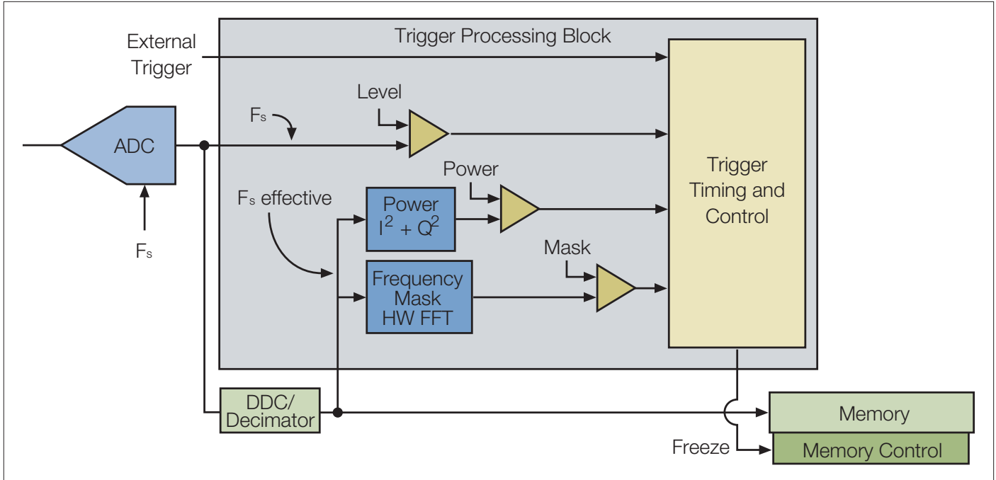
Figure 2-29. Real-Time Spectrum Analyzer trigger processing.
