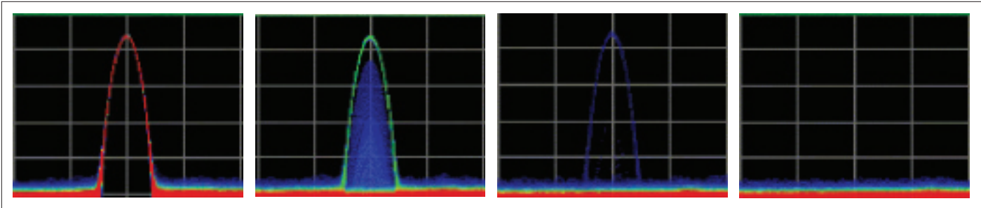
Figure 2-24. With variable persistence, a brief CW signal captured by DPX remains in the display for an adjustable period of time before fading away.
