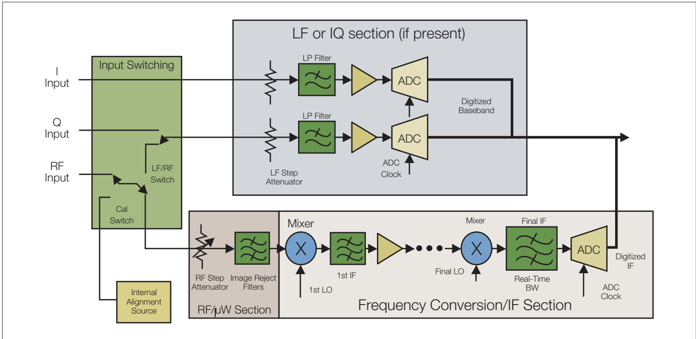
Figure 2-1. Real-Time Spectrum Analyzer RF/IF block diagram.
