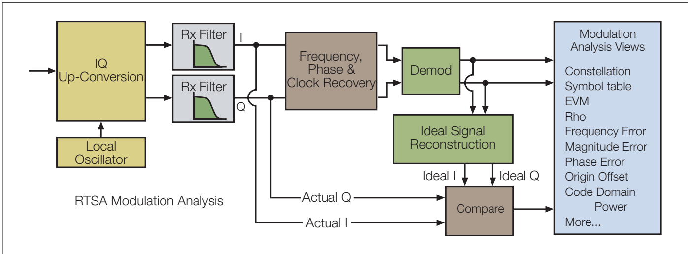
Figure 2-35. RTSA modulation analysis block diagram.
