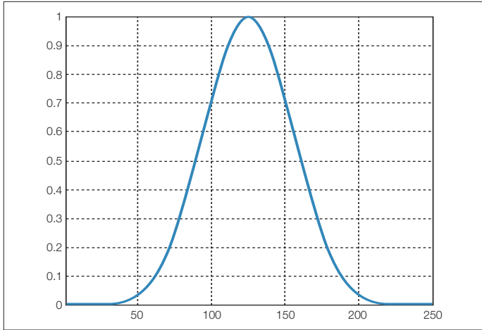
Figure 2-9. Kaiser Window (beta 16.7) in Time Domain (Horizontal is time sample, Vertical is linear scale).
