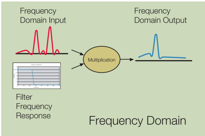
Figure 2-17. Multiplying a filter by its frequency response.
