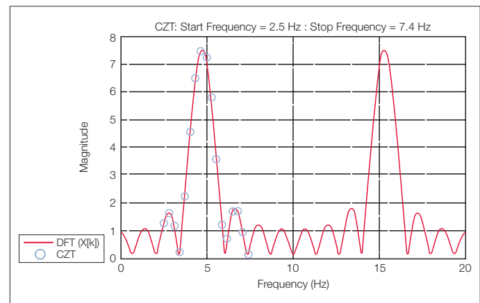
Figure 2-14. CZT of x(n) .
