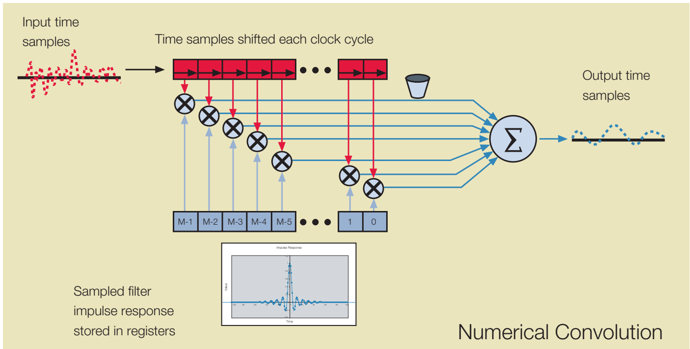
Figure 2-19. Discrete Time Numerical Convolution.
