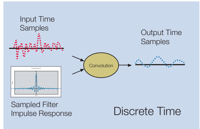
Figure 2-18. Convolution in the time domain is equivalent to multiplication in the frequency domain.
