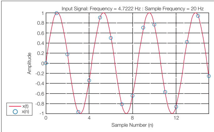
Figure 2-11. Input Signal.
