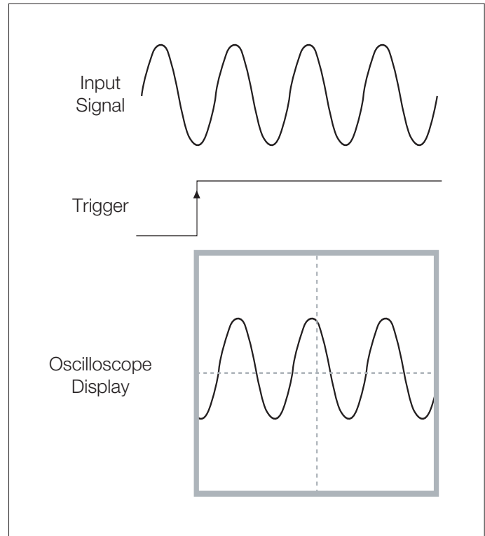
Figure 2-27. Traditional oscilloscope triggering.
