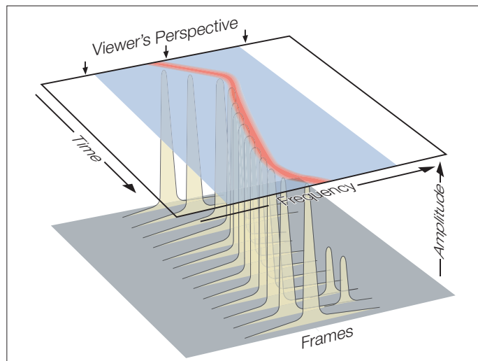
Figure 3-2. Spectrogram display.
