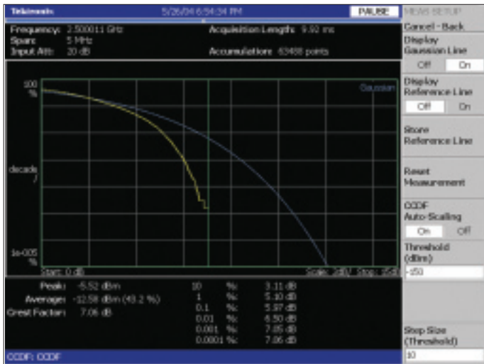
Figure 3-21. CCDF measurement.
