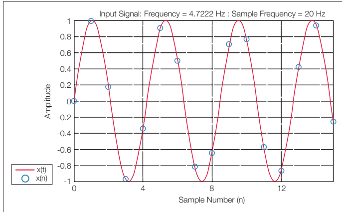
Figure 2-11. Input Signal.
