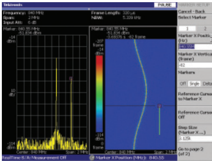
Figure 3-3. Time-correlated views: Power vs. Frequency display (left) and spectrogram display (right).
