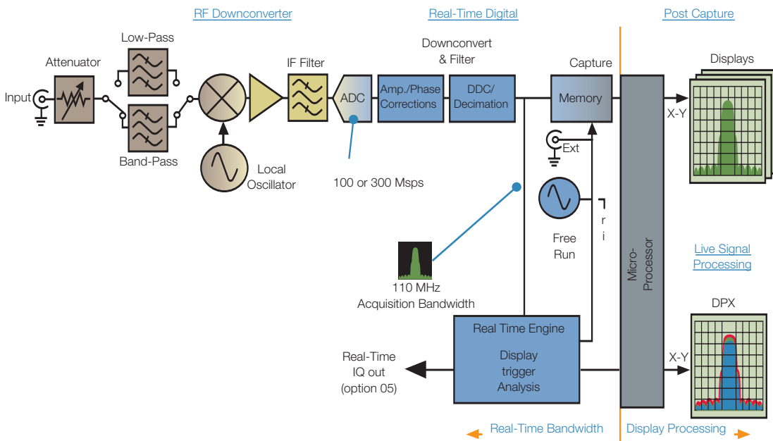
c) Real-Time Spectrum Analyzer (RSA6100 Series + Option 110)
