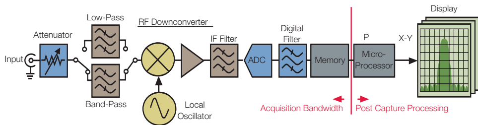
b) Vector Signal Analyzer (VSA)
