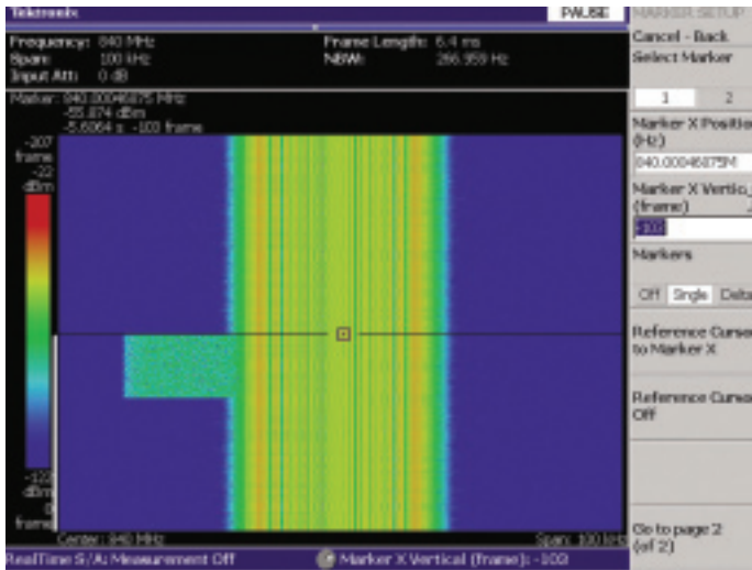
Figure 2-31. Spectrogram showing a transient signal adjacent to the carrier. The cursor is set to the trigger point, so pre-trigger data is displayed above the cursor line, and post-trigger data is displayed below the cursor line. The narrow white line at the left of the blue area denotes post-trigger data.
