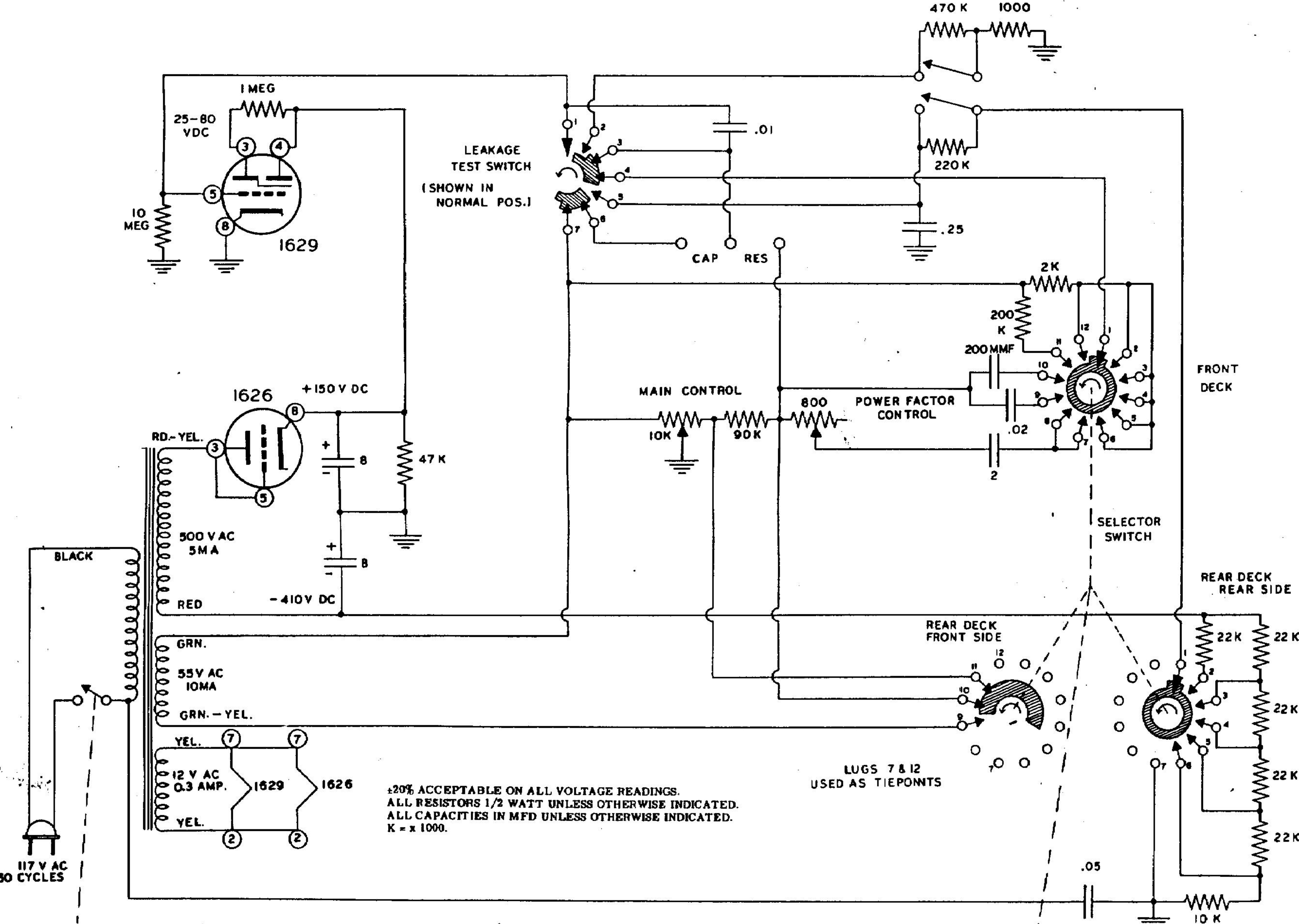
HEATHKIT CONDENSER CHECKER Model C-3
