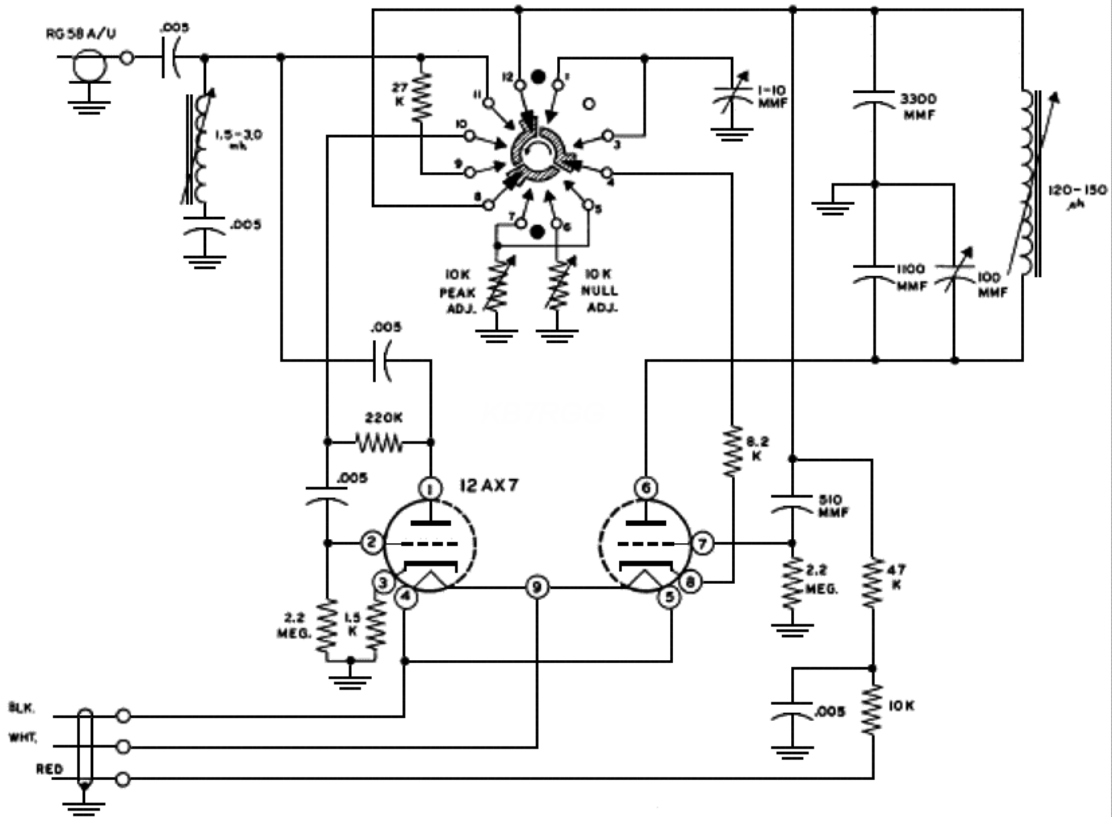
SCHMATIC OF Q MULTIPLIER QF-1
