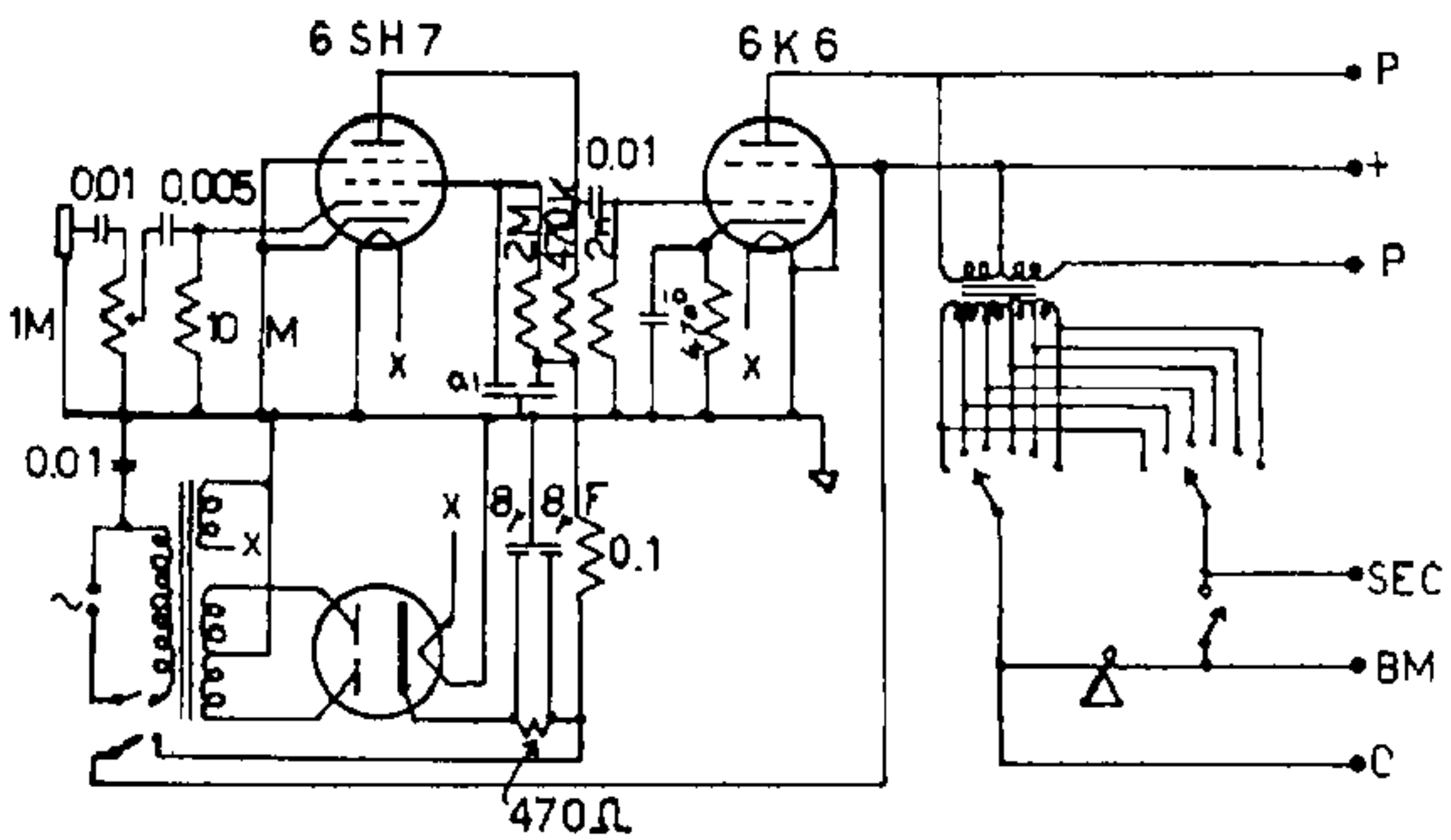
Heathkit signal tracer, mod. T 2
